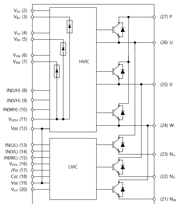
Figure 1. Internal Circuit
