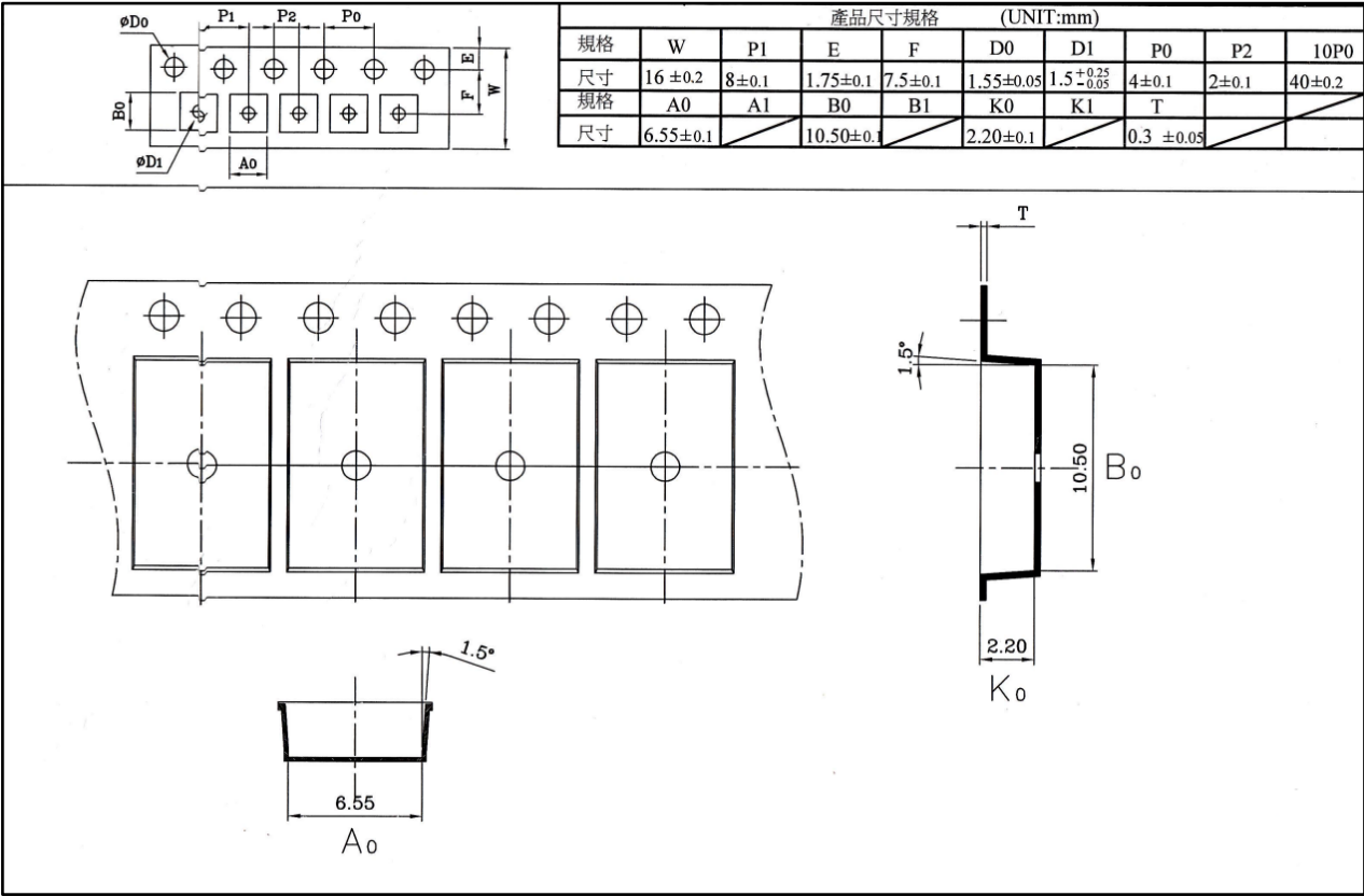
Figure 18. CMT826X NB SOIC-16 Tape and Reel Information
