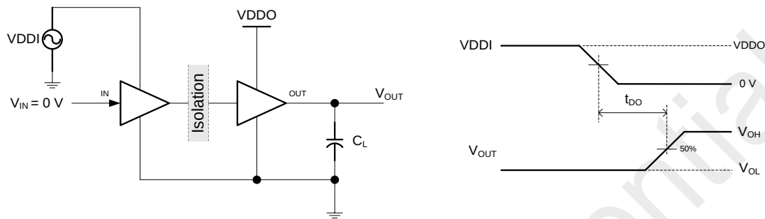
Figure 4. Default Output Delay Time Test Circuit and Voltage Waveforms
