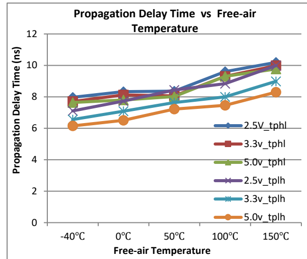
Figure 9-6. Propagation Delay Time vs. Free-Air Temperature
