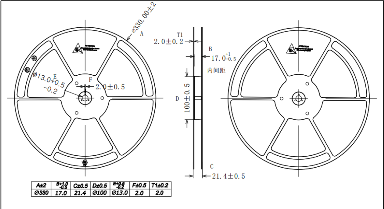
Figure 15. CMT826X WB SOIC-16 Tape and Reel Information
