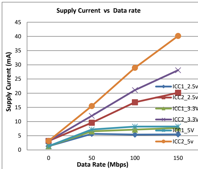
Figure 9-1. Supply Current vs. Data Rate (with 15-pF load) T_A=25^{\circ}\text{C} C_L=15\text{pF}
