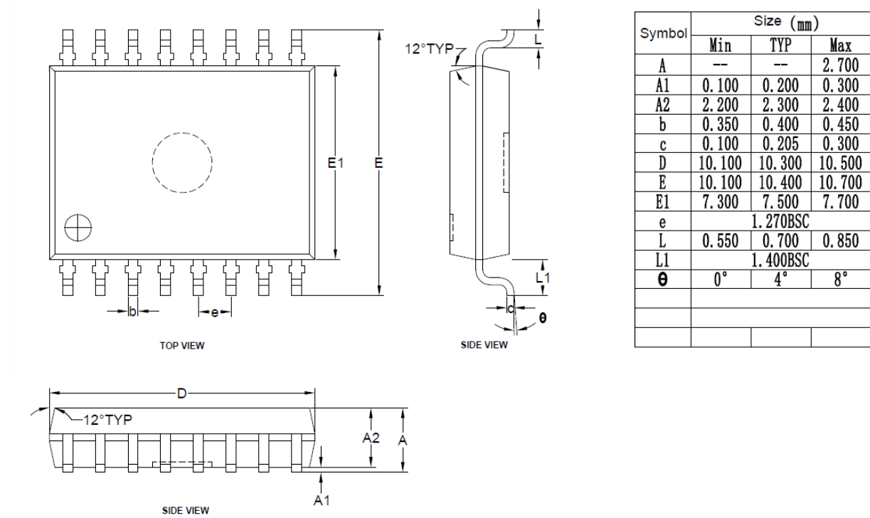
Figure 9. Wide Body SOIC-16 Packaging
