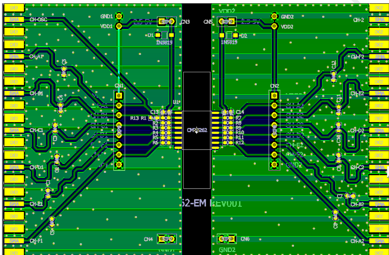
Figure 2. Recommended PCB Layout
