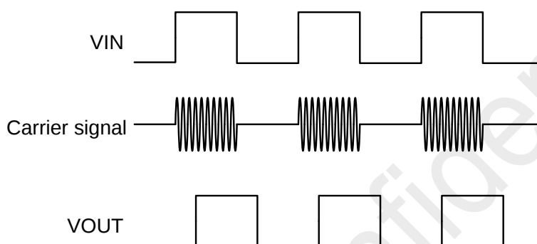
Figure 6. On-Off Keying Based Modulation Scheme
