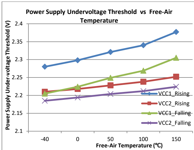
Figure 9-5. Power Supply Under-voltage Threshold vs. Free-Air Temperature
