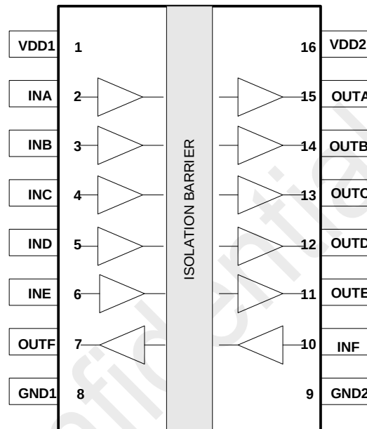
Figure 2. CMT8261 Pin List
