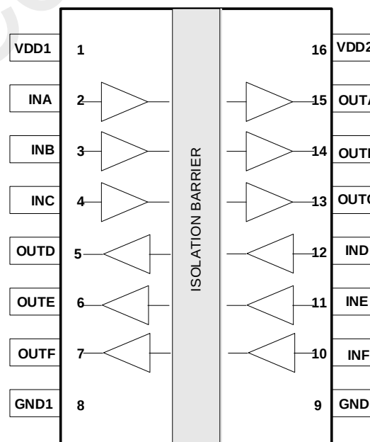
Figure 4. CMT8263 Pin List
