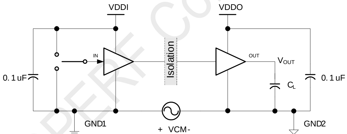
Figure 5. Common-Mode Transient Immunity Test Circuit
