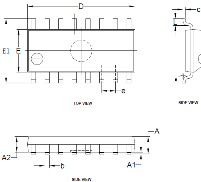
Figure 8. Narrow Body SOIC-16 Packaging
