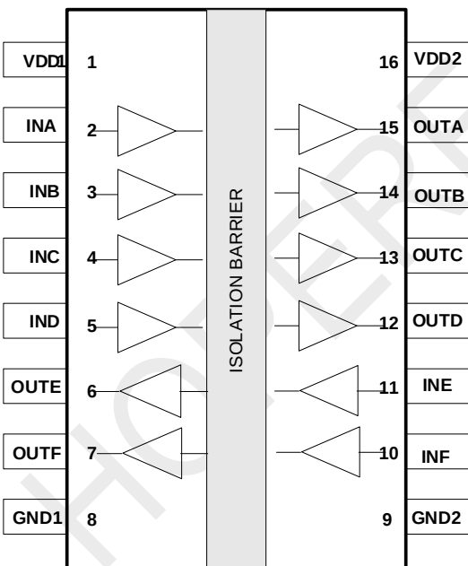
Figure 3. CMT8262 Pin List
