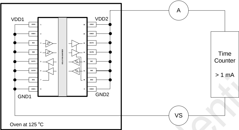
Figure 7. Test Setup for Insulation Lifetime Measurement
