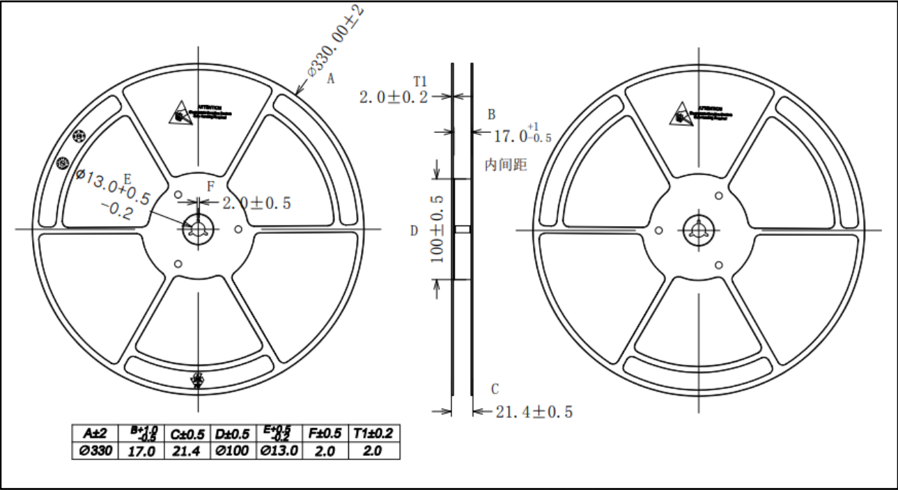
Figure 16. CMT804X NB SOIC-16 Tape and Reel Information
