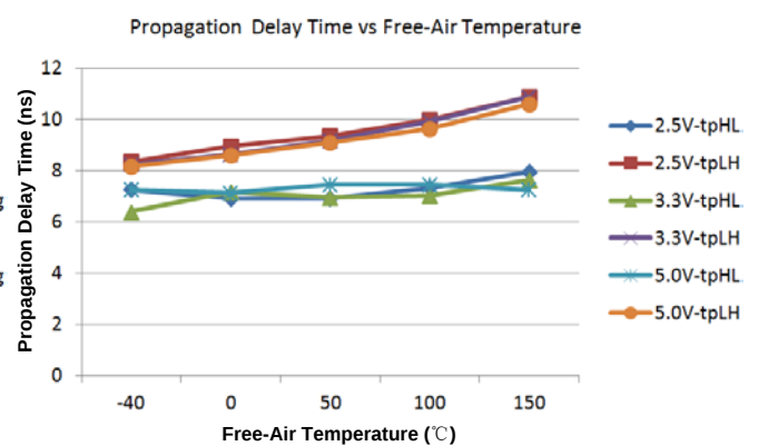
Figure 9-6. Propagation Delay Time vs. Free-Air Temperature
