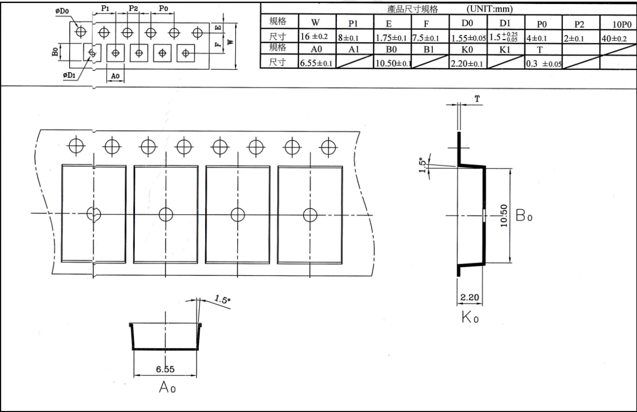
Figure 17. CMT804X NB SOIC-16 Tape and Reel Information
