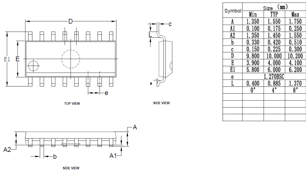
Figure 12. Narrow Body SOIC-16 Packaging
