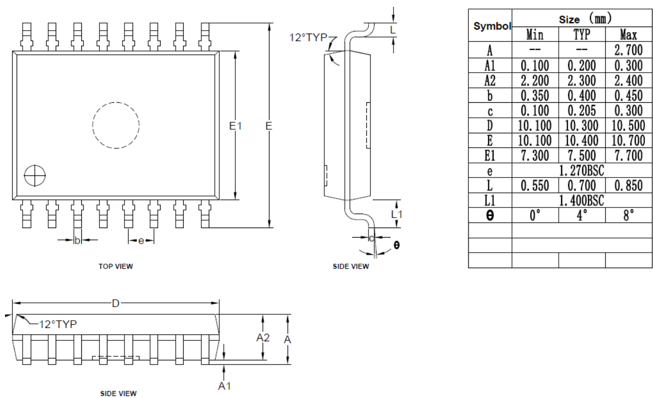
Figure 13. Wide Body SOIC-16 Packaging
