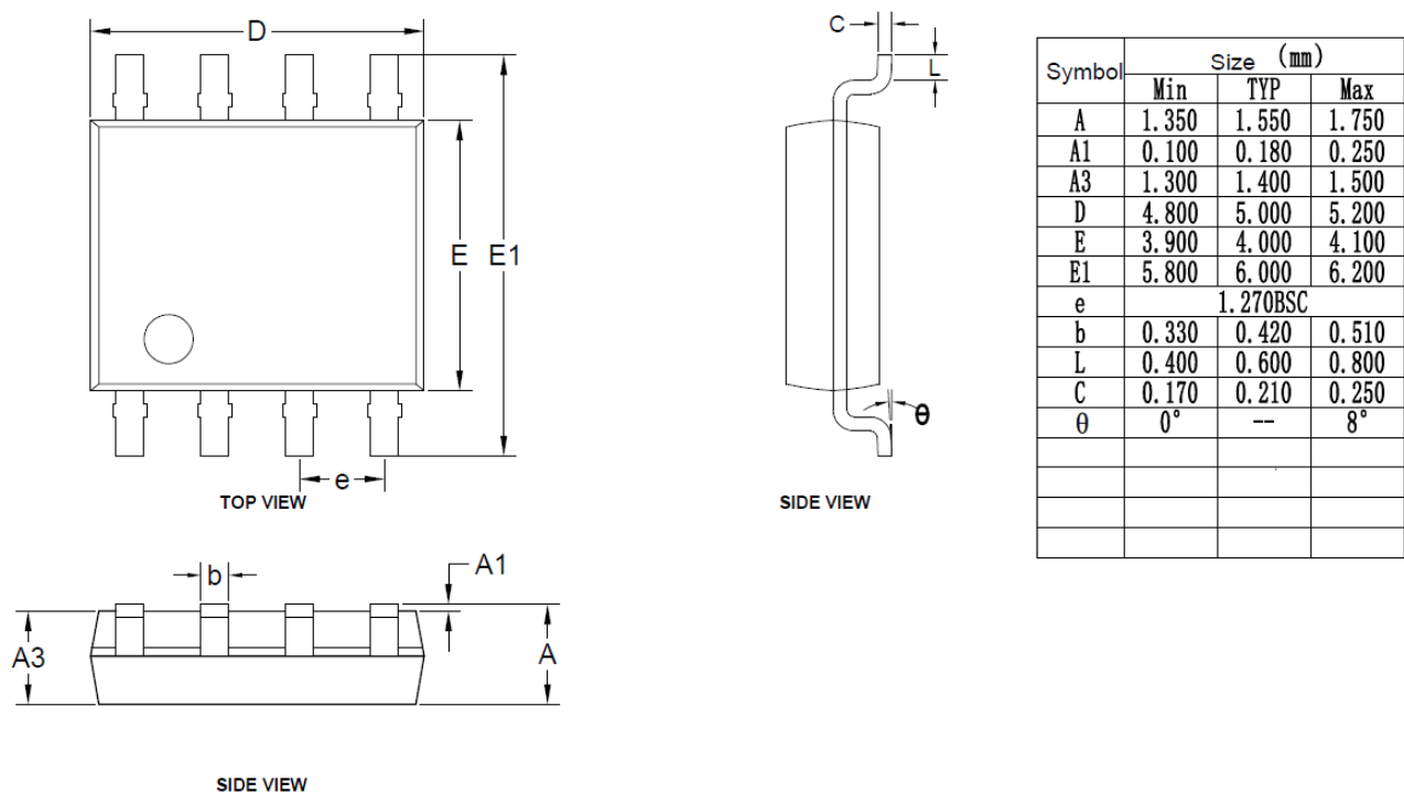
Figure 10. Narrow Body SOIC-8 Packaging
