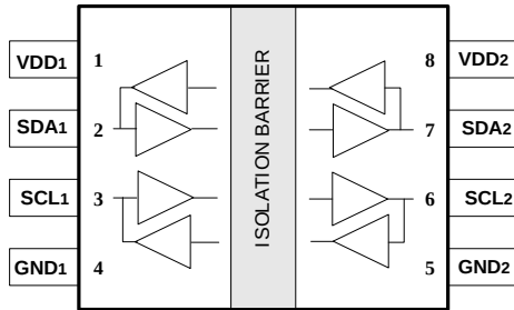
Figure 1. CMT8100N Pin List of SOIC-8 NB/ SOW-8 WB
