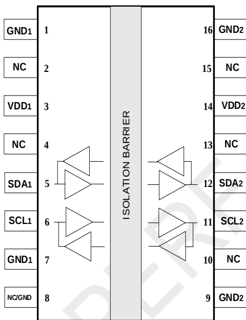
Figure 3 CMT8100W SOIC-16 Pin List
