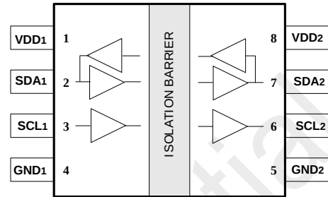
Figure 2. CMT8101N Pin List of SOIC-8 NB/ SOW-8 WB
