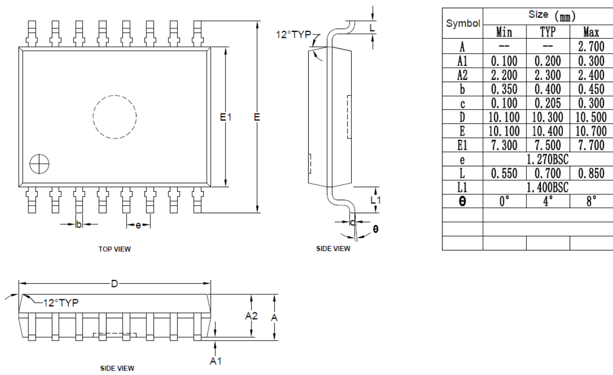
Figure 11. Wide Body SOIC-16 Packaging
