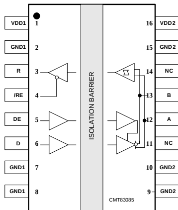
Figure 1-1. CMT83085 Pin List
