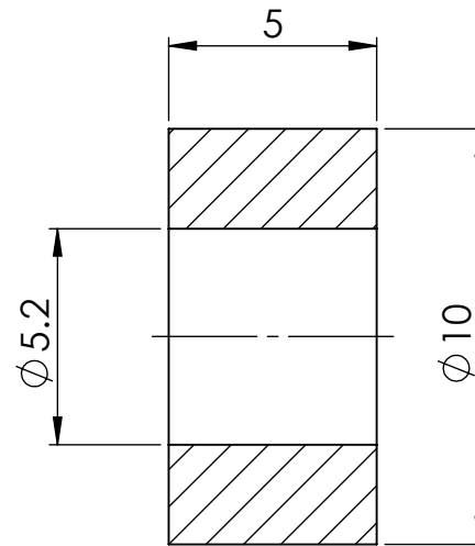
SECTION Y-Y
