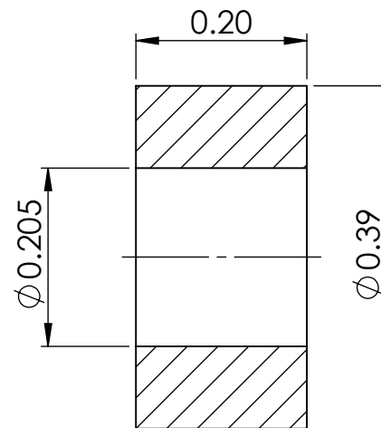
SECTION Y-Y
