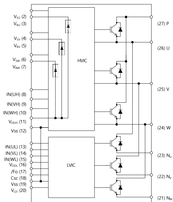
Figure 1. Internal Circuit
