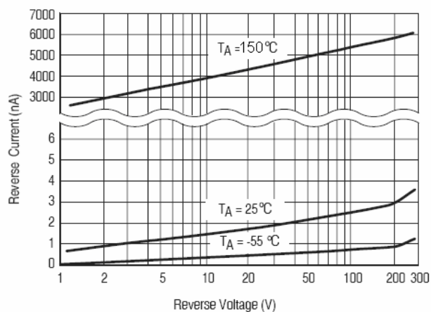
Figure 2. Reverse Leakage
