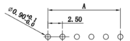
Recommended P.C.Board Hole Layout
