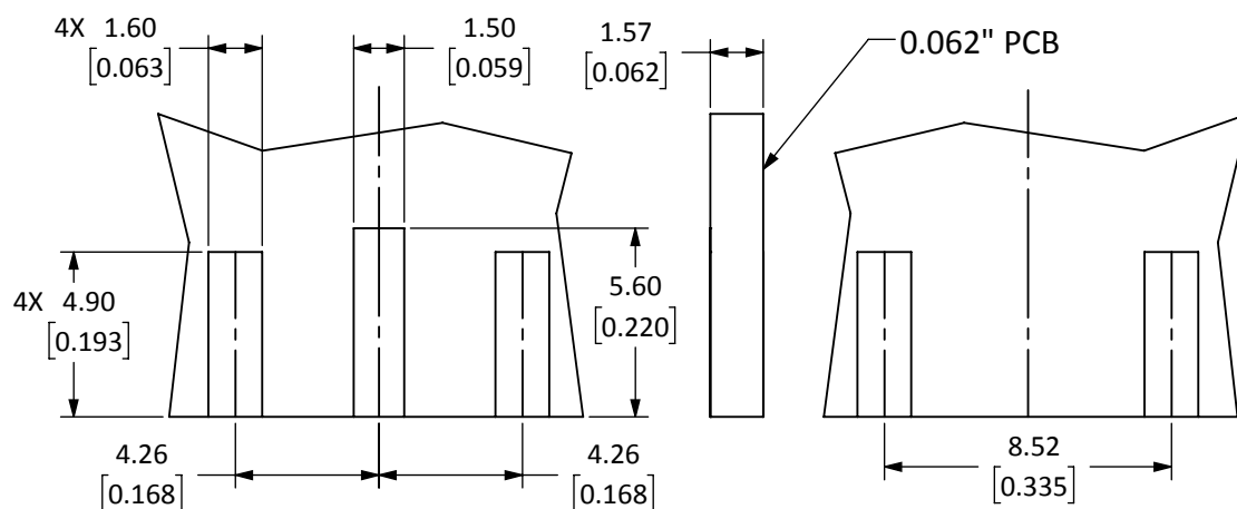
RECOMMENDED FOOTPRINT
