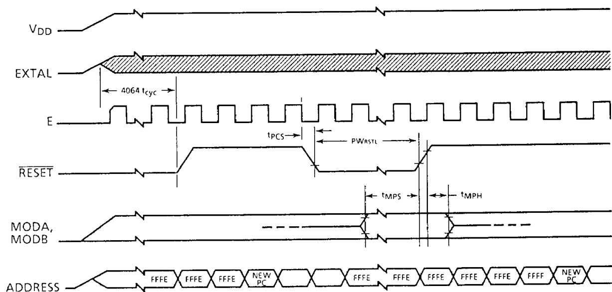
Figure 11.3 POR and External Reset Timing Diagram
