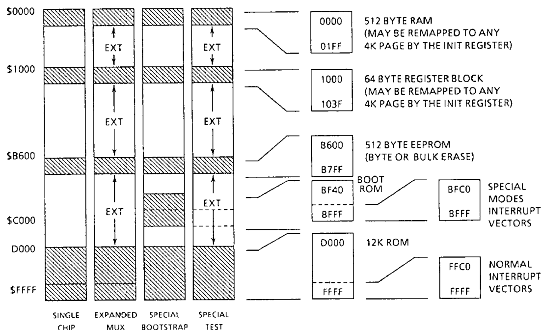
Figure 3.1 Memory Maps
