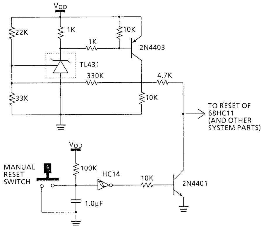
Figure 9.2 Reset Circuit with LVI and RC Delay
