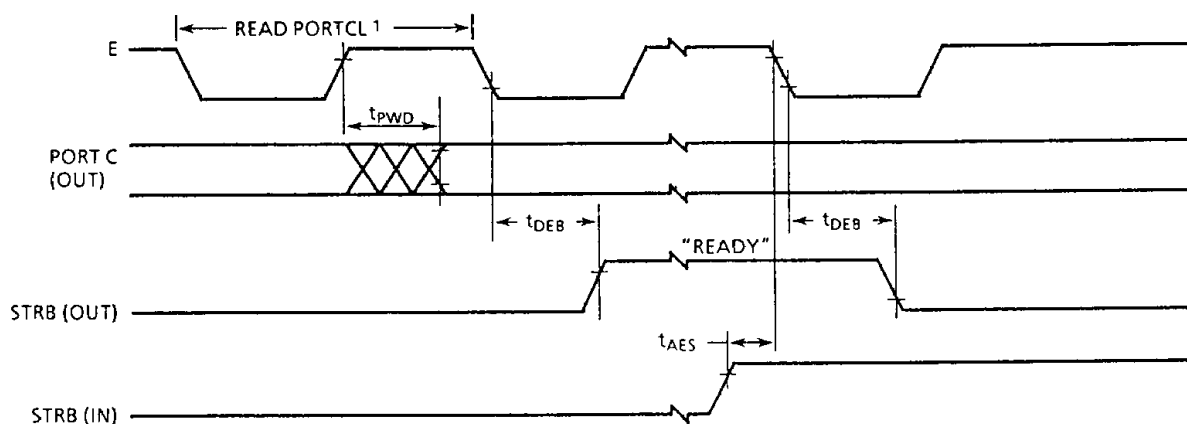
Figure 11.11 Port C Input Handshake Timing Diagram
